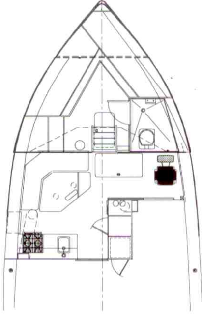
WHEELHOUSE/FORECASTLE PLAN
