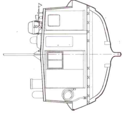
WHEELHOUSE SECTION
